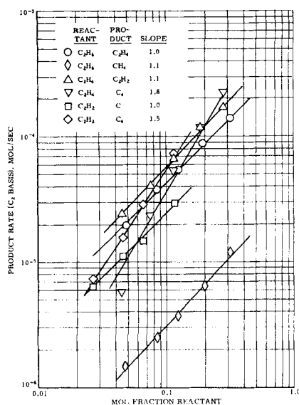
Fig. 4. Orders of reaction.
