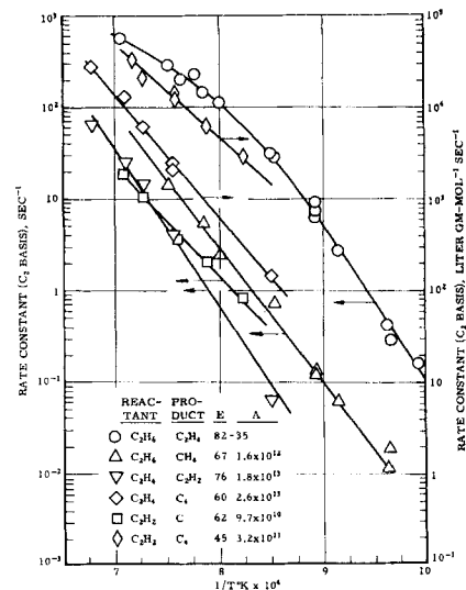
Fig. 6. Rate constants.
