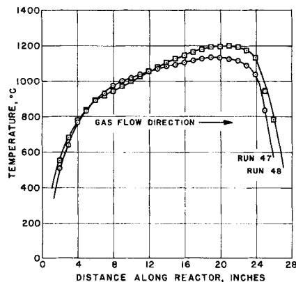
Fig. 5. Temperature profiles.
